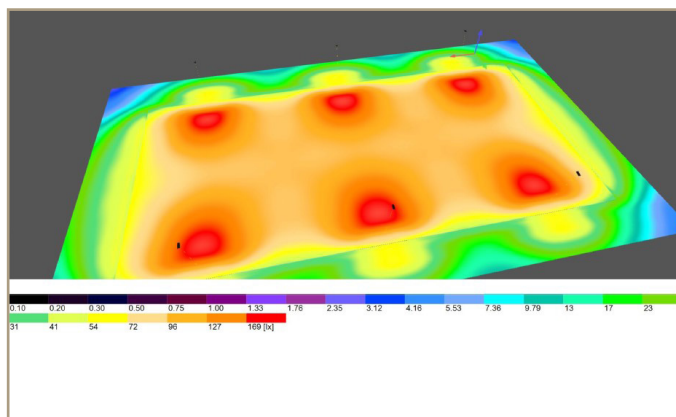
6 projectors in total on 10 m high masts.
