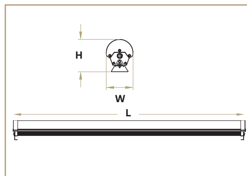
PROXI-BARN-T Model
